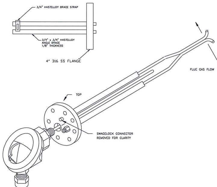
PITOT & THERMOCOUPLE SUPPORT ASSEMBLY
